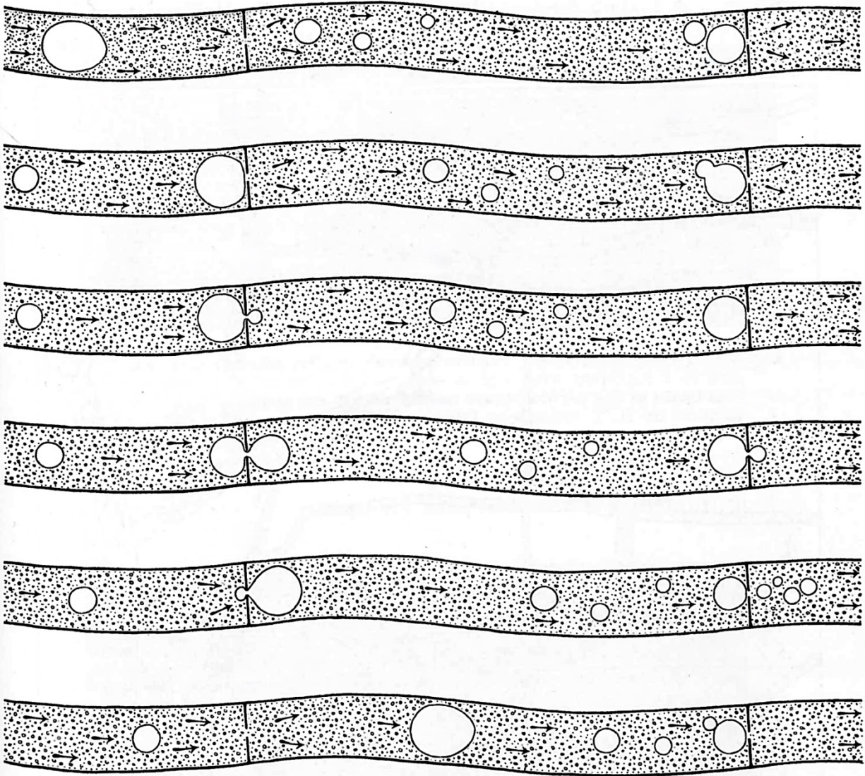
Figure 4. Mass flow of cytoplasm within hyphae from left to right, showing fluid-filled vacuoles squeezing through pores in septa. Successive images of hyphae from top to bottom of the figure are separated by 10 seconds. Source: Adapted from Buller (1933).
