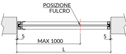
Iris con cerniera decentrata, muro a vista Iris with decentralized hinge, exposed wall
