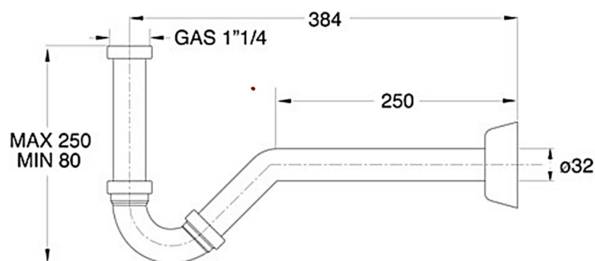
SIFONE "TORINO" Ø32x1"1/4 (2600T25K)
