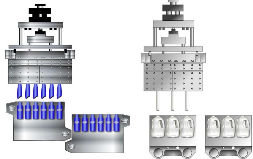
Inclined Carriage
