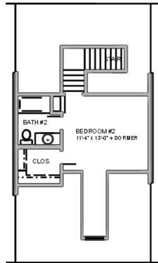
THIRD FLOOR PLAN (UPPER LEVEL OF TOWNHOMES)
