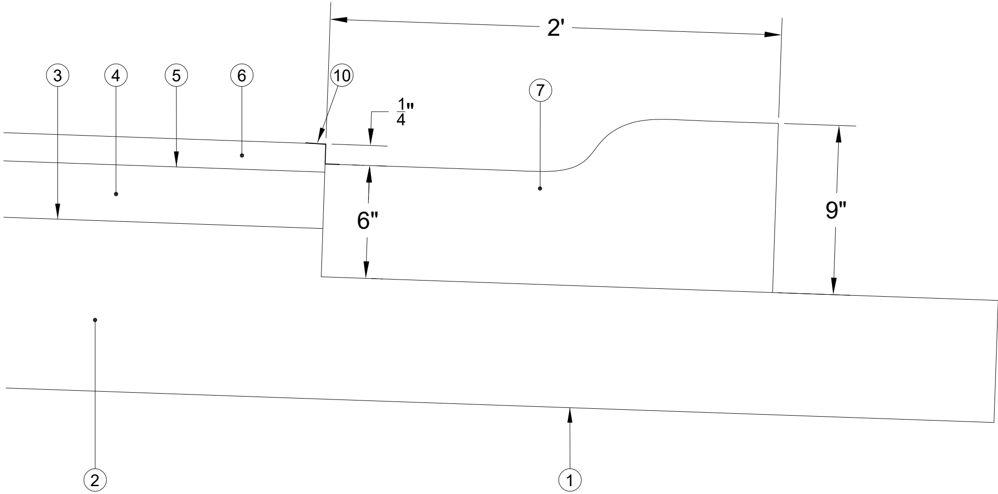
MOUNTABLE CURB DETAIL SCALE: NTS
