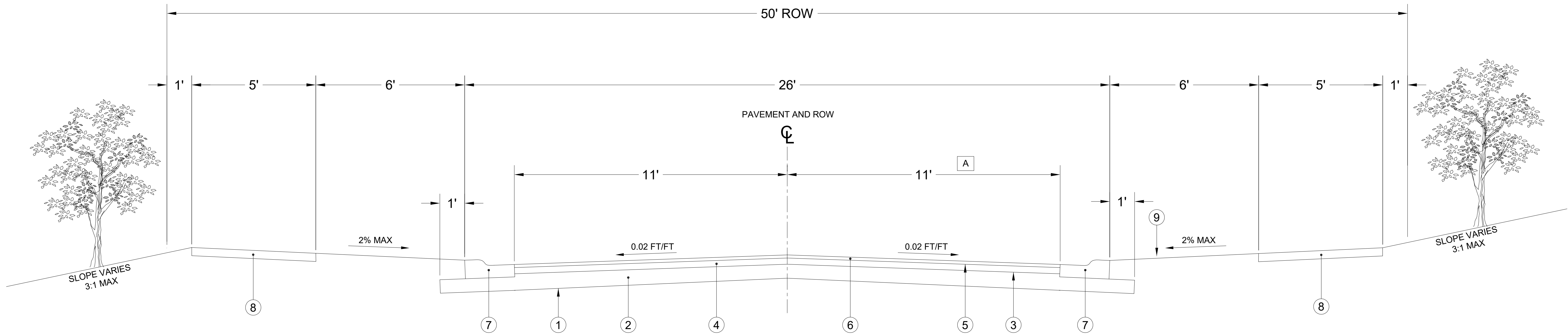
TYPICAL SECTION SCALE: NTS
