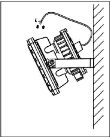
No.2: Wall Mounting
