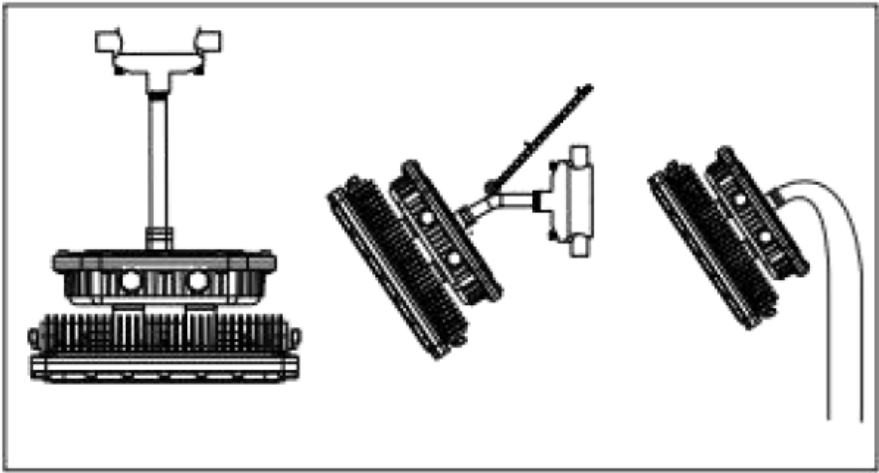
No.3: Pole Mounting
