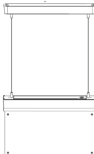
Suspended Chain With Decorative Cover Installation
