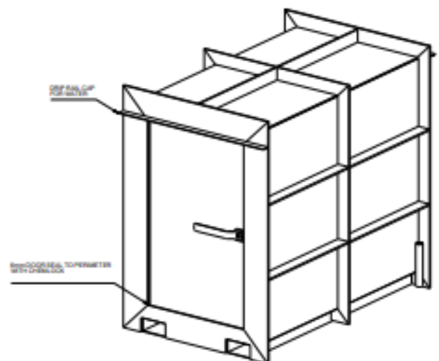
3D VIEW DOOR OPENS IN AND LEFT
