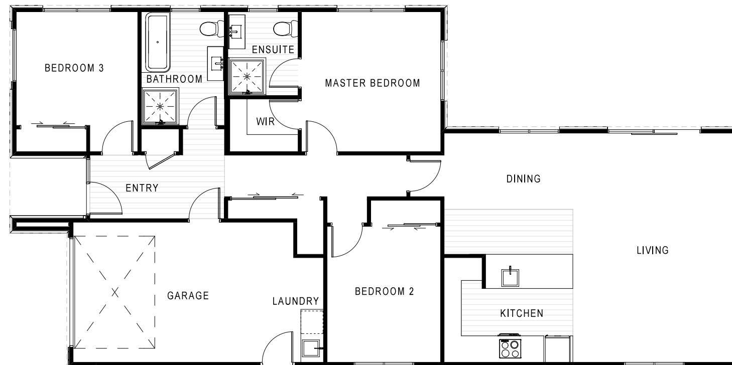
FLOOR PLAN FLOOR AREA: 147m2 over foundation
