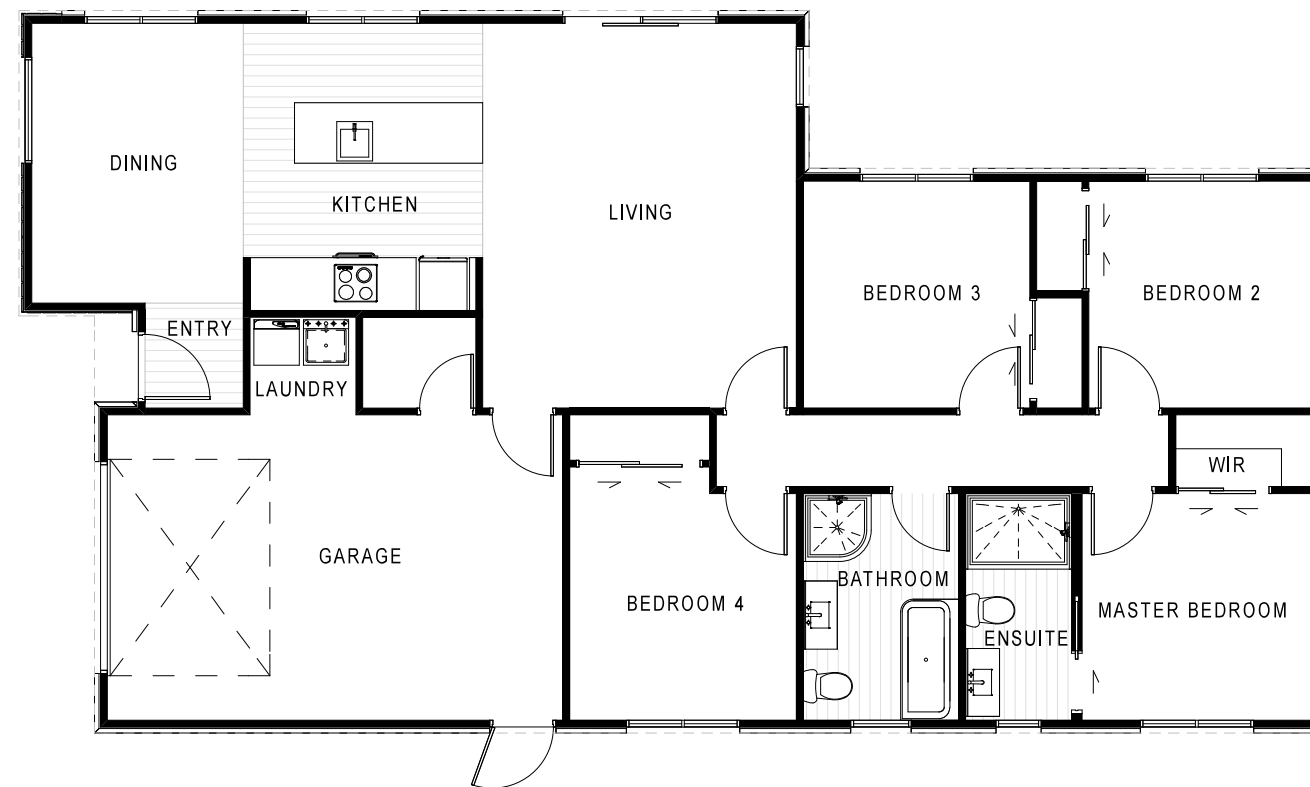
FLOOR PLAN FLOOR AREA: 140.8m2 over foundation
