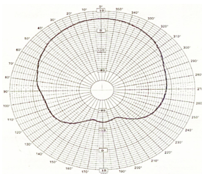
Horizontal Plane Pattern (vertical polarization)
