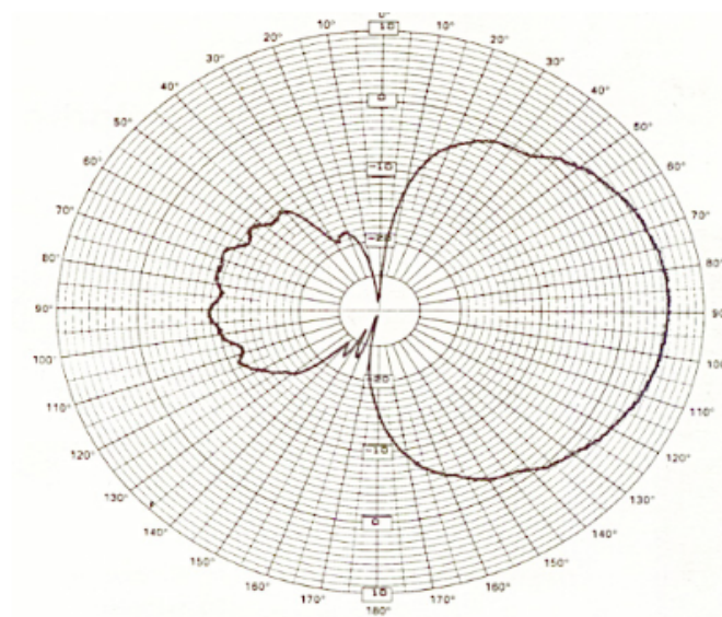
Vertical Plane Pattern (vertical polarization)
