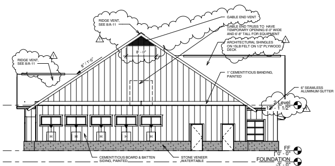
3 REAR 1/8" = 1'-0"
