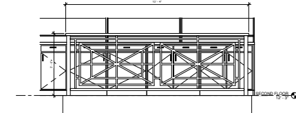
DECORATIVE RAILING DETAIL
