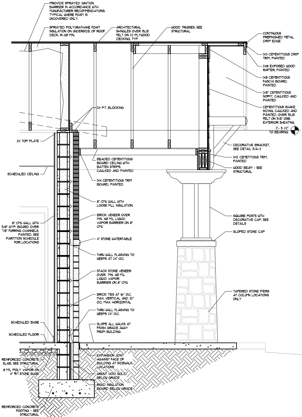
SECTION
