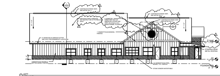
2 LEFT 1/8" = 1'-0"
