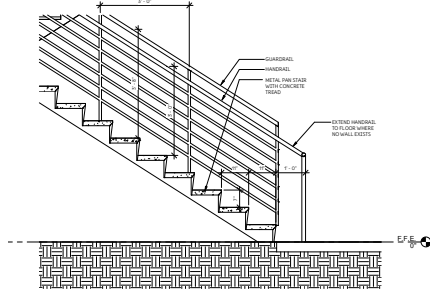
STAIR SECTION
