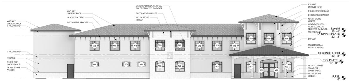
FRONT ELEVATION
