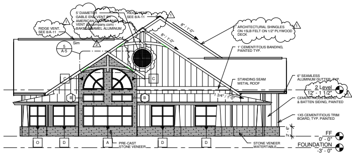
1 FRONT 1/8" = 1'-0"
