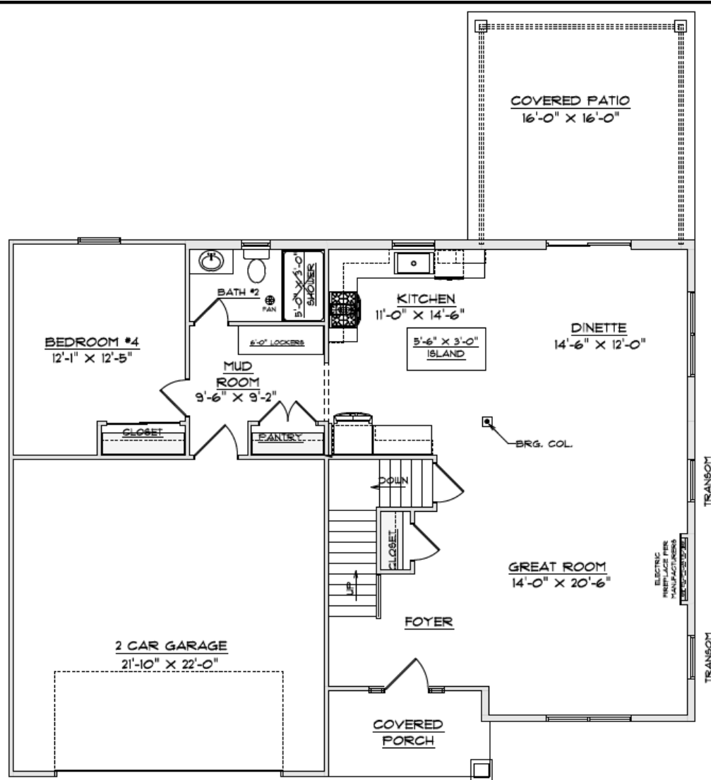
FIRST FLOORPLAN
