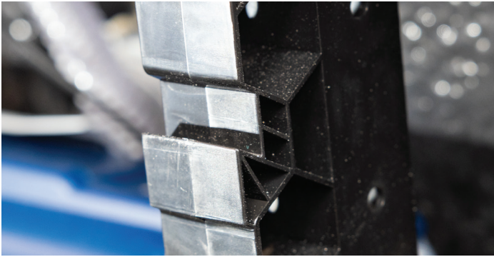
French Cleat (top) and C-Clip (bottom)
