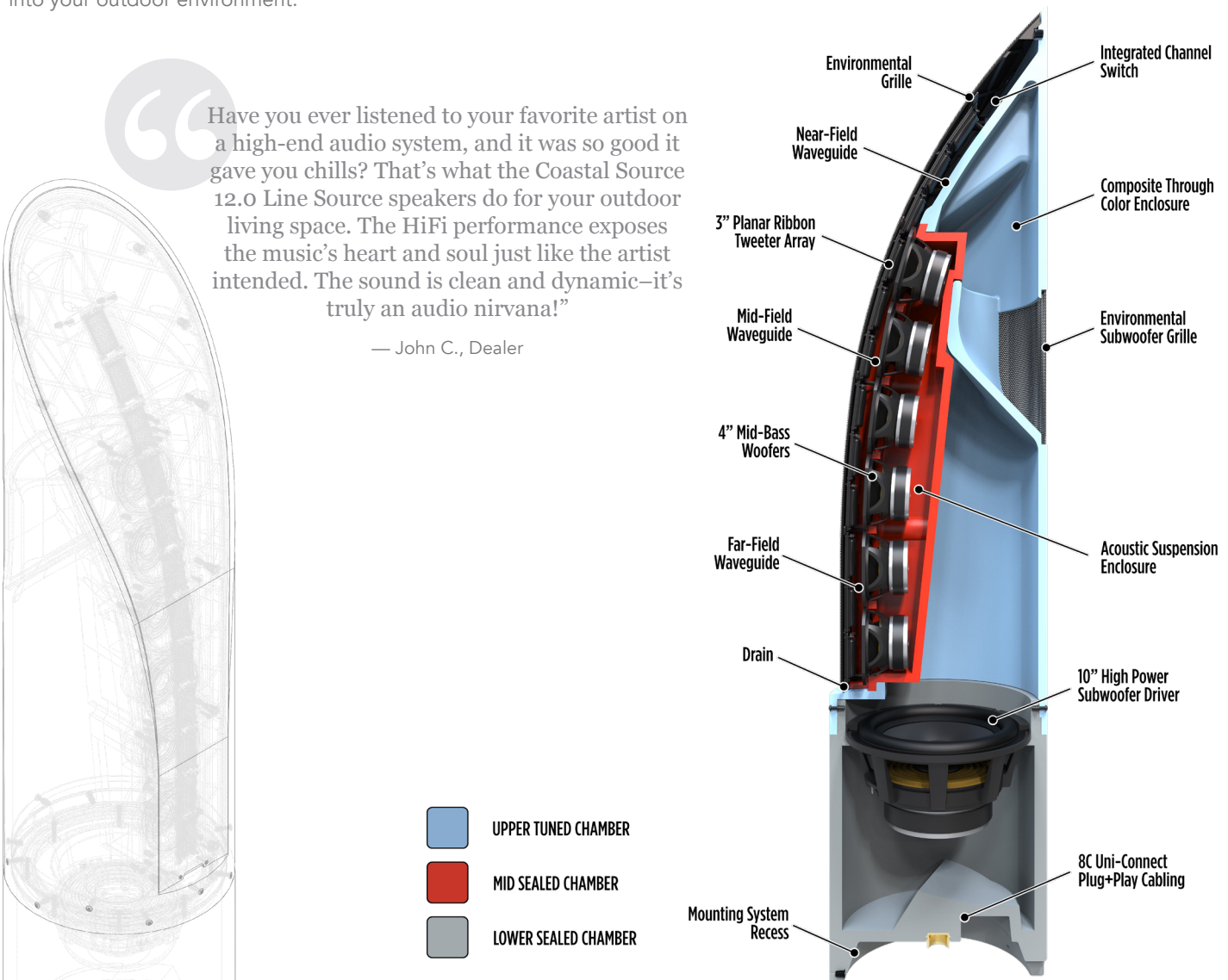
CROSS SECTION OF THE PATENTED 12.0 LINE SOURCE BOLLARD
