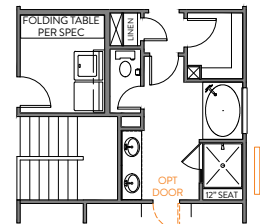
LUXURY BATH 3 42"x60" GARDEN TUB w/CERAMIC TUB SURROUND 42"x48" FRAMED TILE SHOWER BASE TILE WALLS w/12" TILE SEAT
