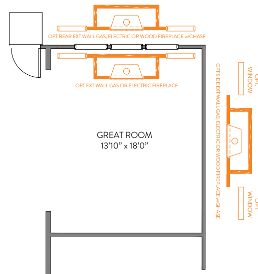
GREAT ROOM FIREPLACE OPTIONS
