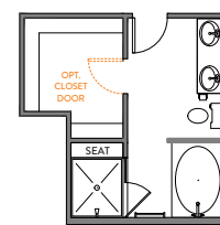
LUXURY BATH 3 42" x 60" GARDEN TUB w/CERAMIC TUB SURROUND 42" x 48" FRAMED TILE SHOWER TILE WALLS w/12" TILE SEAT
