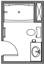
SHOWER BATH 3
