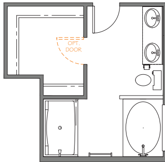
LUXURY BATH OPT. 1 42"x60" Garden Tub 36"x60" Fiberglass Shower Unit
