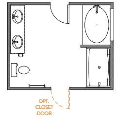
LUXURY BATH 1 42"x60" GARDEN TUB 36"x60" FIBERGLASS SHOWER UNIT REDUCES PRIMARY SUITE BY 2'
