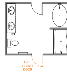
LUXURY BATH 1 42"x60" GARDEN TUB 36"x60" FIBERGLASS SHOWER UNIT REDUCES PRIMARY SUITE BY 2'
