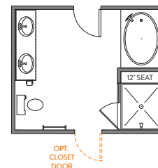
LUXURY BATH 3 42"x60" GARDEN TUB w/CERAMIC TUB SURROUND 42"x48" FRAMED TILE SHOWER BASE TILE WALLS w/12" TILE SEAT REDUCES PRIMARY SUITE BY 2'
