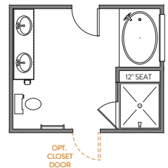
LUXURY BATH 3 42"x60" GARDEN TUB w/CERAMIC TUB SURROUND 42"x48" FRAMED TILE SHOWER BASE TILE WALLS w/12" TILE SEAT REDUCES PRIMARY SUITE BY 2'
