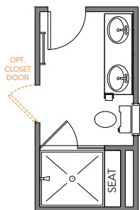
LUXURY SHOWER 2
