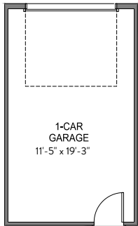
1 CAR DETACHED GARAGE
