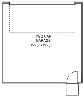
2 CAR DETACHED GARAGE
