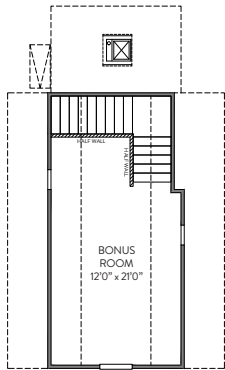
STANDARD BONUS ROOM
