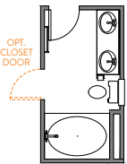
GARDEN TUB/SHOWER LOSE 4" FROM PRIMARY SUITE
