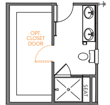
LOSE 12" FROM PRIMARY SUITE
