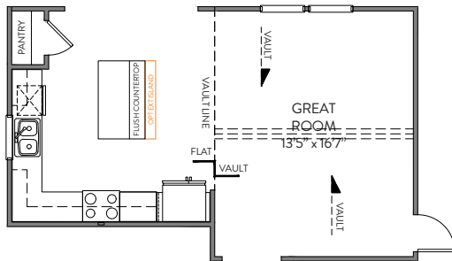
GREAT ROOM VAULTED CEILING
