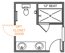
LUXURY SHOWER 36"x60" FRAMED SHOWER PAN TILE WALLS w/12" SEAT FRAMELESS SHOWER DOOR
