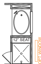
LUXURY BATH 3 42"X60" GARDEN TUB w/CERAMIC TUB SURROUND 42"X48" FRAMED TILE SHOWER BASE TILE WALLS w/12" TILE SEAT
