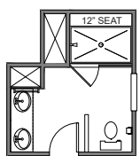
LUXURY SHOWER 36"x60" FRAMED PAN TILE WALLS w/12" SEAT FRAMELESS SHOWER DOOR
