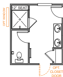
LUXURY SHOWER 2 42\"/>
