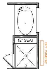
LUXURY BATH 3 42"x60" GARDEN TUB w/CERAMIC TUB SURROUND 42"x48" FRAMED TILE SHOWER BASE TILE WALLS w/12" TILE SEAT
