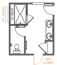
LUXURY SHOWER 36\"/>
