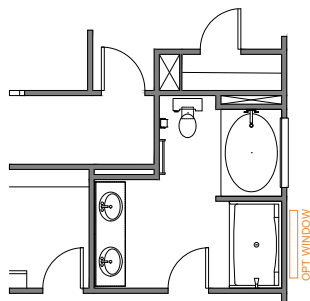
LUXURY BATH 1 42"x60" GARDEN TUB 35"x60" FIBERGLASS SHOWER UNIT
