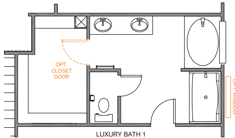
LUXURY BATH 1 42"x60" GARDEN TUB 35"x60" FIBERGLASS SHOWER UNIT
