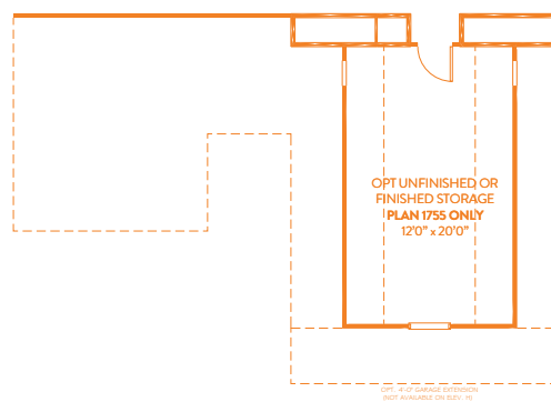
OPT UNFINISHED/FINISHED STORAGE AREA 2 PLAN 1755 ALT GUEST SUITE NA w/H ELEVATIONS
