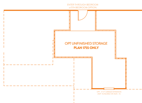
OPT UNFINISHED STORAGE AREA 1 PLAN 1755 ALT GUEST SUITE
