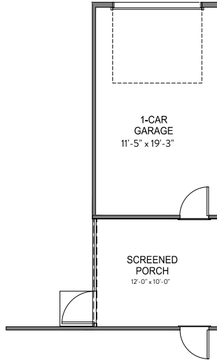
1 CAR GARAGE w/SCEENED PORCH OPT SIDE WALL GREAT ROOM WINDOWS STD. w/THIS OPTION
