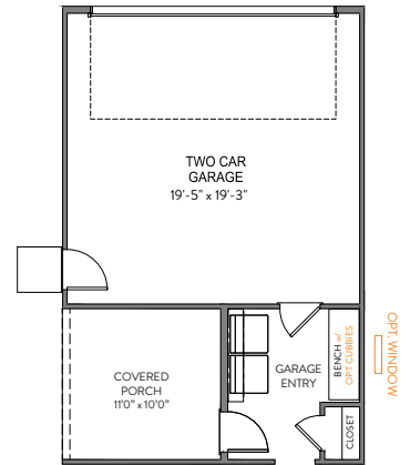
2 CAR GARAGE w/COVERED PORCH AND LAUNDRY ROOM OPT SIDE WALL GREAT ROOM WINDOWS STD. w/THIS OPTION
