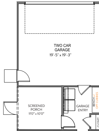
2 CAR GARAGE w/SCREENED PORCH AND LAUNDRY ROOM OPT SIDE WALL GREAT ROOM WINDOWS STD. w/THIS OPTION
