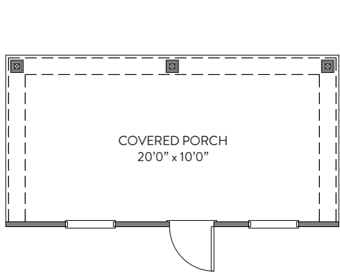
COVERED PORCH
