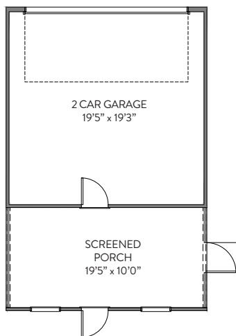
2 CAR GARAGE w/SCREENED PORCH OPT SIDE WALL GREAT ROOM WINDOWS STD. w/THIS OPTION
