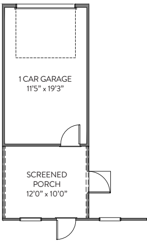
1 CAR GARAGE w/COVERED PORCH OPT SIDE WALL GREAT ROOM WINDOWS STD. w/THIS OPTION
