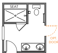
LUXURY SHOWER 36"X60" FRAMED PAN TILE WALLS w/12" TILE SEAT FRAMELESS SHOWER DOOR
