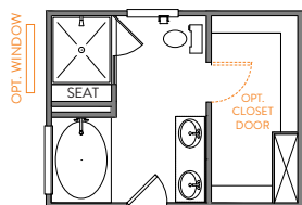
LUXURY BATH 3 42"X60" GARDEN TUB w/CERAMIC TUB SURROUND 42"X48" FRAMED TILE SHOWER BASE TILE WALLS w/12" TILE SEAT TAKES 11" FROM PRIMARY SUITE
