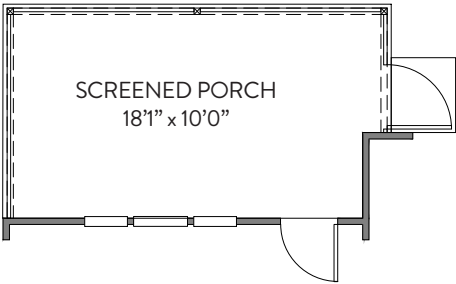
SCREENED PORCH
