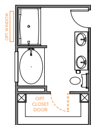
LUXURY BATH 1 42"x60" GARDEN TUB 35"x60" FIBERGLASS SHOWER UNIT
