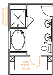
LUXURY BATH 3 42"x60" GARDEN TUB W/CERAMIC TUB SURROUND 42"x42" FRAMED TILE SHOWER BASE TILE WALLS W/12" TILE SEAT
