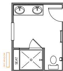
LUXURY SHOWER 2 42"x48" FRAMED SHOWER PAN TILE WALLS W/12" SEAT
