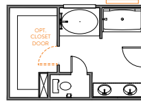
LUXURY BATH 1 42"x60" GARDEN TUB 35"x60" FIBERGLASS SHOWER UNIT
