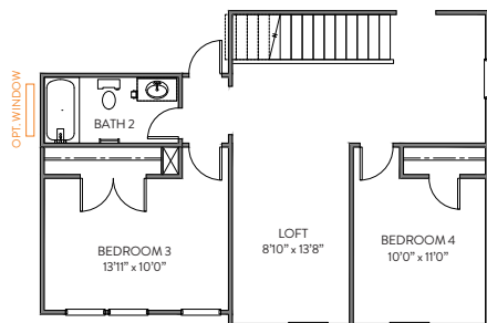
BEDROOM 4 OPTION REPLACES BONUS ROOM
