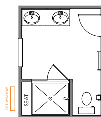
LUXURY SHOWER 2 42"x48" FRAMED SHOWER PAN TILE WALLS W/12" SEAT
