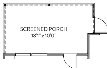
SCREENED PORCH ALT KITCHEN 1 & 2
