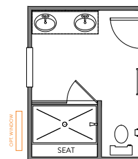
LUXURY SHOWER 36"x60" FRAMED PAN, TILE WALLS w/12" SEAT FRAMELESS SHOWER DOOR
