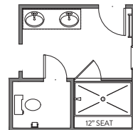
LUXURY SHOWER 36"x60" FRAMED PAN TILE WALLS W/12" SEAT FRAMELESS SHOWER DOOR
