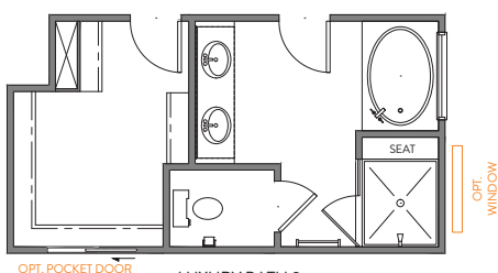
LUXURY BATH 3 42"x60" GARDEN TUB w/CERAMIC TUB SURROUND 42"x48" FRAMED TILE SHOWER BASE TILE WALLS w/12" TILE SEAT
