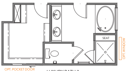
LUXURY BATH 3 42"x60" GARDEN TUB w/CERAMIC TUB SURROUND 42"x48" FRAMED TILE SHOWER BASE TILE WALLS w/12" TILE SEAT
