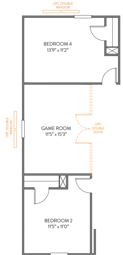
Opt. Second Floor 2 w/Bump Second Floor Plan E, F, H, L Elevations w/4'5" Bump Adds 53 sq ft
