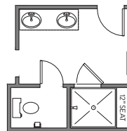
LUXURY SHOWER OPT. 2 42"x48" FRAMED TILE SHOWER BASE TILE WALLS W/12" SEAT
