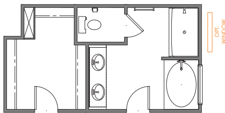
LUXURY BATH 1 42"x60 GARDEN TUB 35"x60" FIBERGLASS SHOWER UNIT
