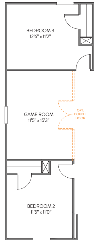
Opt. Second Floor 1 w/Bump Second Floor Plan E, F, H, L Elevations w/4'5" Bump Adds 53 sq ft
