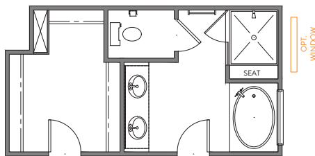
LUXURY BATH 3 42"x60" GARDEN TUB w/CERAMIC TUB SURROUND 42"x48" FRAMED TILE SHOWER BASE TILE WALLS w/12" TILE SEAT
