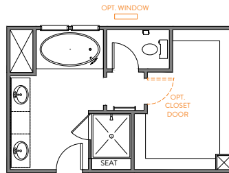
LUXURY BATH OPTION 6 42" x 72" GARDEN TUB w/CERAMIC TUB SURROUND 42" x 48" FRAMED TILE SHOWER BASE TILE WALLS w/12" TILE SEAT LOSE CUBBY
