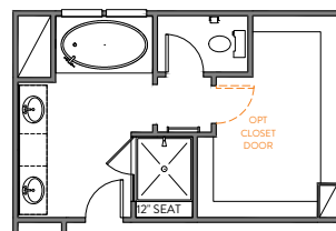
LUXURY BATH OPTION 6 42" X 72" GARDEN TUB w/CERAMIC TUB SURROUND 42" X 48" FRAMED TILE SHOWER BASE TILE WALLS w/12" TILE SEAT
