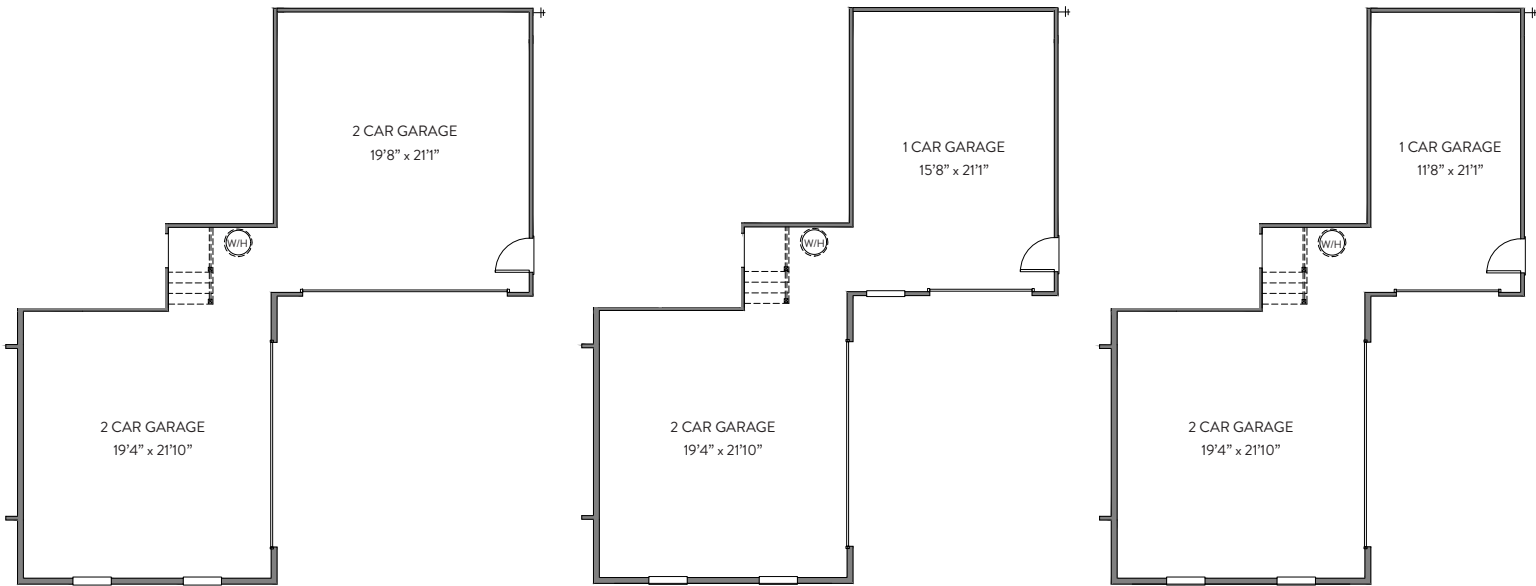
4 CAR COURTYARD GARAGE OPT 3
