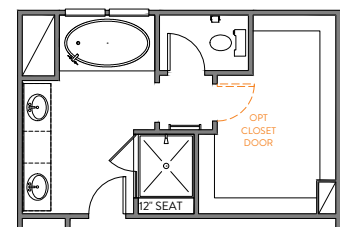
42" X 72" GARDEN TUB w/CERAMIC TUB SURROUND 42" X 48" FRAMED TILE SHOWER BASE TILE WALLS w/1/2" TILE SEAT
