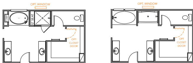
LUXURY BATH OPTION 3 42" X 60" GARDEN TUB w/CERAMIC TUB SURROUND 42" X 48" FRAMED TILE SHOWER BASE TILE WALLS w/12" TILE SEAT
