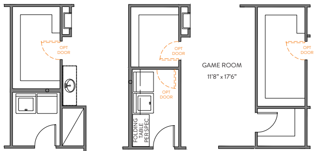
LAUNDRY ROOM OPT 1
