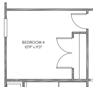
BEDROOM 4 ILO GAME ROOM
