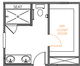
LUXURY SHOWER 36"x60" FRAMED PAN TILE WALLS w/12" SEAT FRAMELESS SHOWER DOOR
