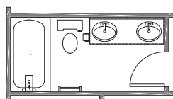
DUAL BOWL VANITY N/A w/GARDEN TUB
