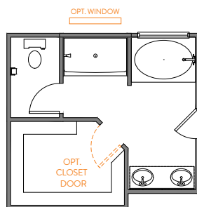
LUXURY BATH 1 35"x60" FIBERGLASS SHOWER UNIT 42"x60" GARDEN TUB REMOVES 12" FROM GAME ROOM/ OPT BEDROOM 4
