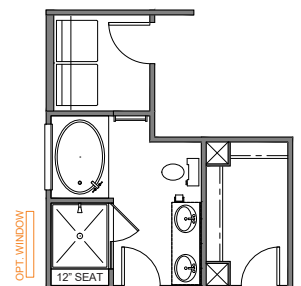
LUXURY BATH 3 42"x60" GARDEN TUB W/CERAMIC TUB SURROUND 42"x48" PRE-FORM SURROUND TILE WALLS w/12" SEAT LOSE 6" FROM PRIMARY CLOSET
