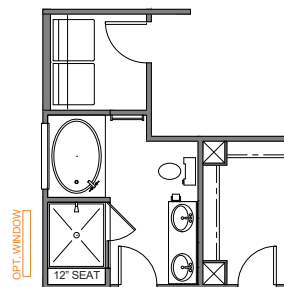
LUXURY BATH 3 42"x60" GARDEN TUB W/CERAMIC TUB SURROUND 42"x48" PRE-FORM SURROUND TILE WALLS w/12" SEAT LOSE 6" FROM PRIMARY CLOSET
