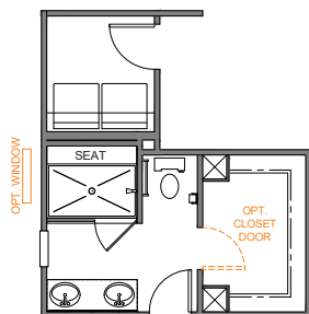
LUXURY SHOWER 36"x60" FRAMED PAN TILE WALLS w/12" TILE SEAT FRAMELESS SHOWER DOOR
