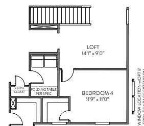
BEDROOM 4 ILO GAME ROOM
