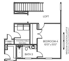
BEDROOM 4 w/FULL BATH ILO GAME ROOM
