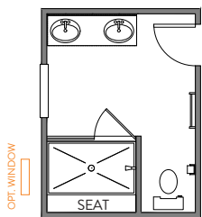
LUXURY SHOWER 36"X60" FRAMED PAN TILE WALLS w/12" TILE SEAT FRAMELESS SHOWER DOOR
