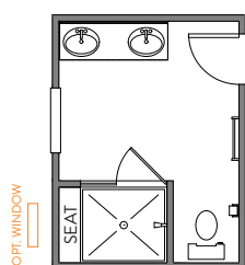
LUXURY SHOWER 2 42"X42" FRAMED PAN TILE WALLS w/12" TILE SEAT FRAMELESS SHOWER DOOR
