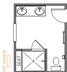
LUXURY SHOWER 2 42"X42" FRAMED PAN TILE WALLS w/12" TILE SEAT FRAMELESS SHOWER DOOR
