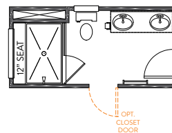
LUXURY SHOWER 36"X60" FRAMED SHOWER PAN TILE WALLS w/12" TILE SEAT FRAMELESS SHOWER DOOR LOSE 9" FROM PRIMARY SUITE LOSE 9" FROM CLOSET
