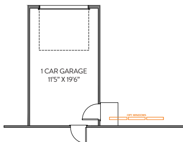
ATTACHED 1 CAR GARAGE
