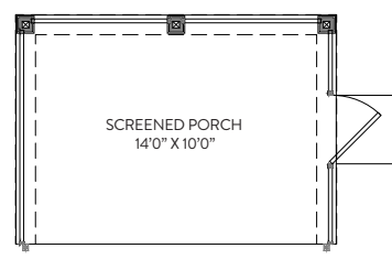
SCREENED PORCH
