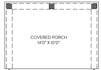
COVERED PORCH
