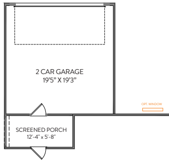
ATTACHED 2 CAR GARAGE W/ SCREENED PORCH 12'-4" X 5'-8"
