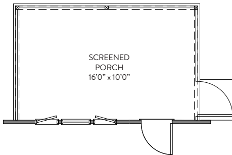
SCREENED PORCH
