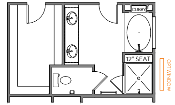
LUXURY BATH OPT 3 42" X 60" GARDEN TUB 42" X 48" TILE PAN 12" TILE SEAT
