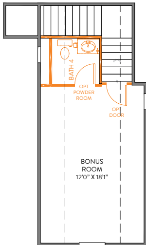
STANDARD ABOVE GARAGE BONUS ROOM w/ OPT POWDER ROOM
