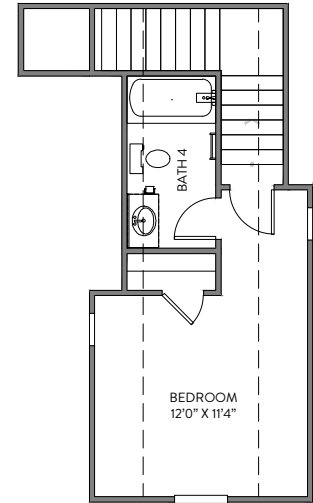
BEDROOM w/FULL BATH
