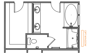
LUXURY BATH OPT 4 42" X 72" GARDEN TUB 34" X 60" FIBERGLASS SHOWER
