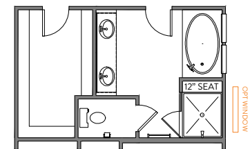
LUXURY BATH OPT 6 42" X 72" GARDEN TUB 42" X 48" TILE PAN 12" TILE SEAT
