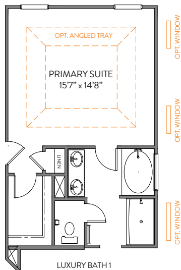
LUXURY BATH 1 42"x60" GARDEN TUB 35"x60" SHOWER TAKES 17 SQ FT FROM WIC ADDS 6" TO PRIMARY SUITE
