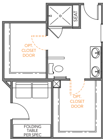
LUXURY SHOWER 2 TAKES 12" FROM WIC AND 12" FROM LAUNDRY
