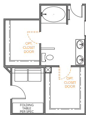
GARDEN TUB/SHOWER
