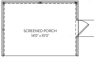
SCREENED PORCH
