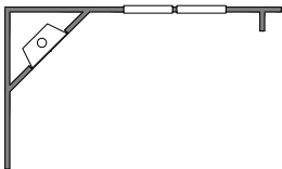
EXT WALL CORNER GAS OR ELECTRIC FIREPLACE
