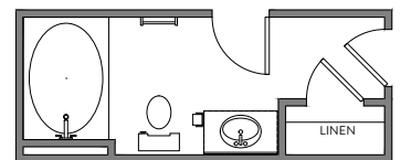
GARDEN TUB/SHOWER
