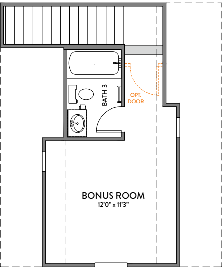
BONUS ROOM w/FULL BATH
