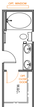
GARDEN TUB/SHOWER (TAKES 6 1/2" FROM THE W.I.C.)
