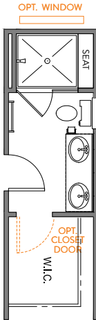
LUXURY SHOWER 2 42" X 48" FRAMED TILE SHOWER BASE TILE WALLS w/12" TILE SEAT (TAKES 6 1/2" FROM THE W.I.C.)
