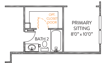
PRIMARY SITTING ROOM
