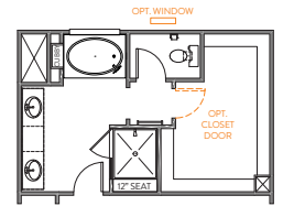
LUXURY BATH OPTION 3 42" X 60" GARDEN TUB w/ CERAMIC TUB SURROUND 42" X 48" FRAMED TILE SHOWER BASE TILE WALLS w/12" TILE SEAT
