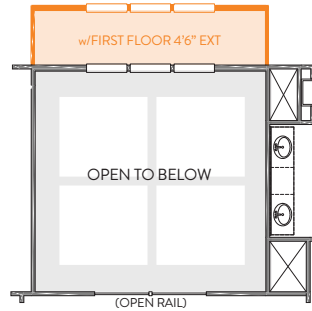
2 STORY GREAT ROOM w/8" DRYWALL BEAMS AND CROWN MOLDING
