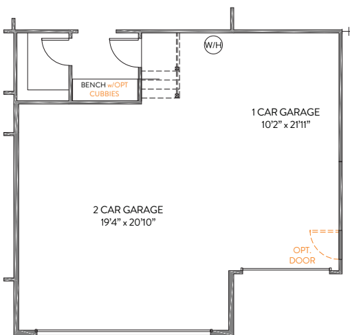
3 CAR FRONT LOAD GARAGE
