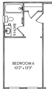
BEDROOM 6 REPLACES LIVING ROOM & LAUNDRY ROOM REQUIRES GARAGE LAUNDRY OR 2ND FLOOR LAUNDRY
