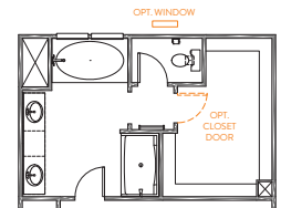
LUXURY BATH OPTION 4 42" X 72" GARDEN TUB 35" X 60" FIBERGLASS SHOWER UNIT
