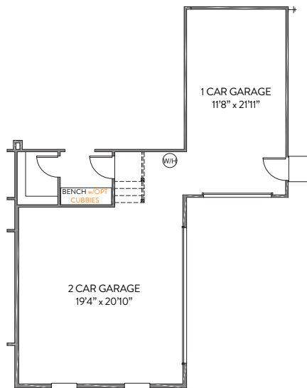
3 CAR COURTYARD GARAGE OPT 1
