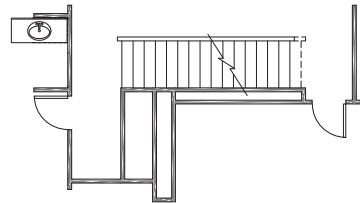
STAIR LOCATION w/OPT 3RD FLOOR
