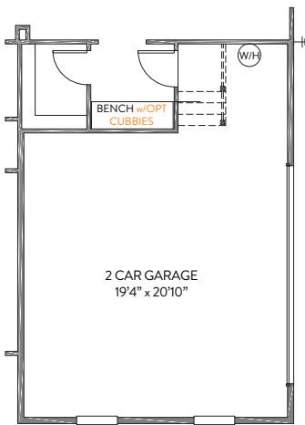
SIDE LOAD GARAGE
