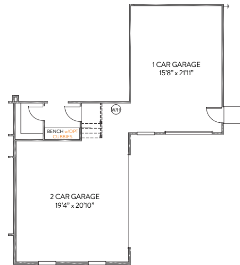
3 CAR COURTYARD GARAGE OPT 2
