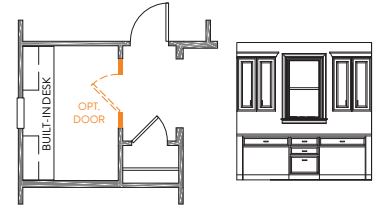
TECHNOLOGY CENTER REQUIRES GARAGE LAUNDRY OR 2ND FLOOR LAUNDRY
