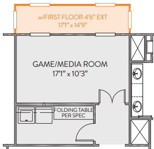
GAME/MEDIA ROOM w/LAUNDRY
