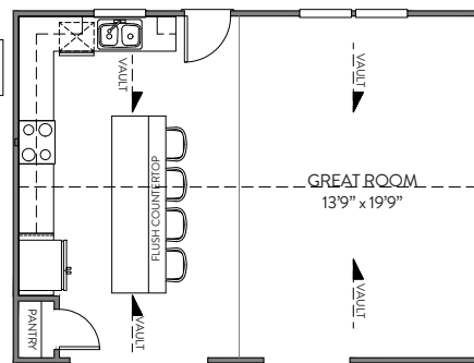
VAULTED CEILING
