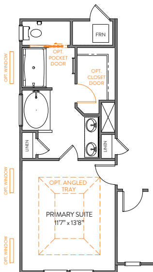
LUXURY BATH 1 42"x60" GARDEN TUB 35"x60" FIBERGLASS SHOWER UNIT
