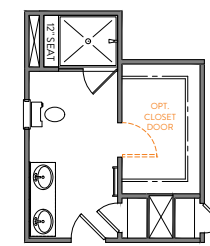
LUXURY SHOWER 2 42"x48" FRAMED TILE SHOWER BASE TILE WALLS W/12" TILE SEAT
